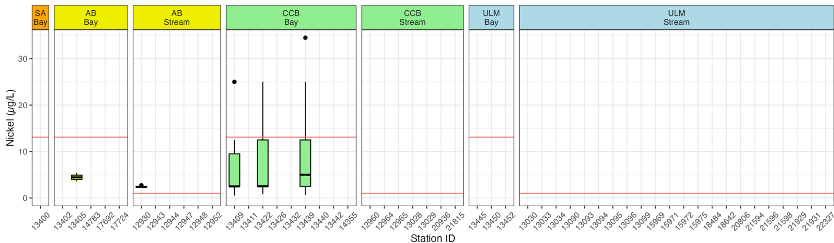
Figure D15. Nickel levels at all stations with available data. The horizontal red line represents the TCEQ screening criteria levels for nickel (13.1 µg/L in bay sites and 0.997 µg/L in stream sites). The high levels shown in Corpus Christi Bay (stations 13409, 13422, and 13439) were due to censored values with an LOD above the screening criteria.
